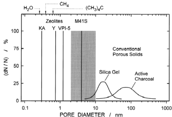
Figure 3: Typical pore diameter distributions of porous solids (KA is the K form of zeolite A; VPI-5 is a microporous aluminophosphate with 18-membered-ring pores; M41S is a family of mesoporous MCM materials). For comparison, the kinetic diameters of water, methane and neopentane are also indicated [reproduced with permission from ref. 107].
