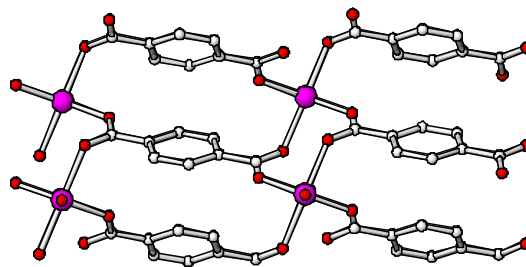
Figure 12: The Zn/DAP/TA structure comprises a 3-D network arising through interconnection of the square-pyramidal Zn units and terephthalate (BDC) ions. Each BDC is coordinated to four Zn atoms (Zn atoms are violet, C atoms grey and O atoms red). Single-crystal data: C 2/c, a=17.9978(5) , b=6.3647(1) , c=7.2657(2) , \beta=91.467(1)^\circ .
