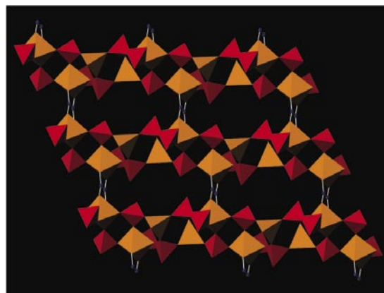
Figure 9: Structure of three-dimensional inorganic-organic (hybrid) framework; Three-dimensional APOX ( [\text{H}_3\text{NCH}(\text{C}_2\text{H}_5)\text{CH}_2\text{NH}_3]_2[\text{Al}_4\text{P}_6\text{O}_{20}(\text{OH})_4(\text{C}_2\text{O}_4)(\text{H}_2\text{O})] ) structure ( \text{PO}_4 tetrahedra are red, the \text{AlO}_4 tetrahedra and \text{AlO}_6 octahedra are orange). The APOX layers are connected through oxalate bridges (C-atoms are shown as blue circles) into a three-dimensional open-framework material. Template molecules are omitted for clarity. Single-crystal data: P-1, a = 8.611(1) \text{ \AA} , b = 9.096(1) \text{ \AA} , c = 11.371(1) \text{ \AA} , \alpha = 104.811(1)^\circ , \beta = 111.368(1)^\circ , and \gamma = 94.248(1)^\circ .
