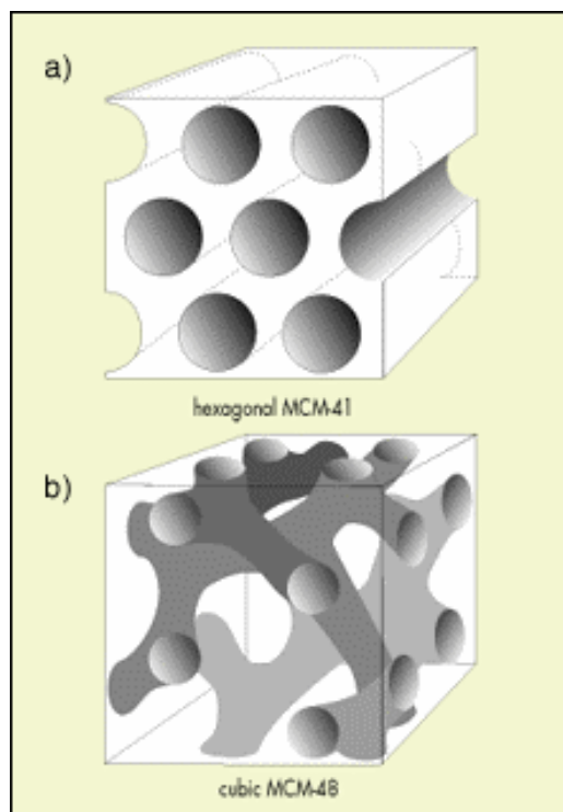
Figure 2: Mesoporous silicates were reported by Mobil Oil scientists in 1992; (a) MCM-41, which stands for Mobil Composition of Matter No. 41, shows a highly ordered hexagonal array of one-dimensional pores with a very narrow pore size distribution. The walls, however, very much resemble amorphous silica. (b) MCM-48 has a cubic mesostructure, i.e. arrangement of the pores.
