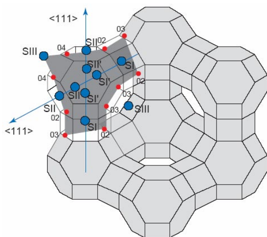
Figure 1: Structure and possible cation sites (SI, SII, etc.) in zeolite faujasite. Due to the presence of aluminium, zeolites exhibit a negatively charged framework, which is counter-balanced by positive cations resulting in a strong electrostatic field on the internal surface. These cations can be exchanged to fine-tune the pore size or the adsorption characteristics [reproduced with permission from ref. 106].
